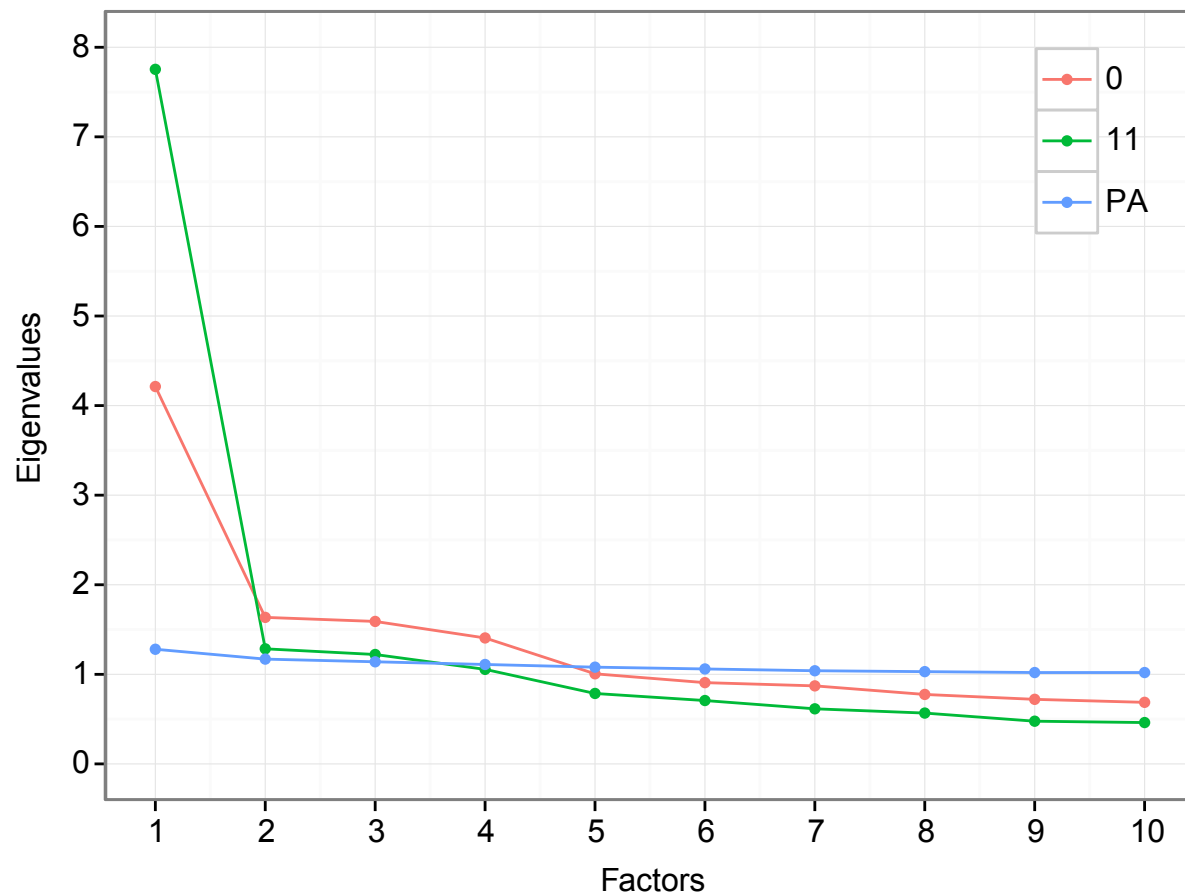
HRSD Eigenvalues at weeks 0 and 11
