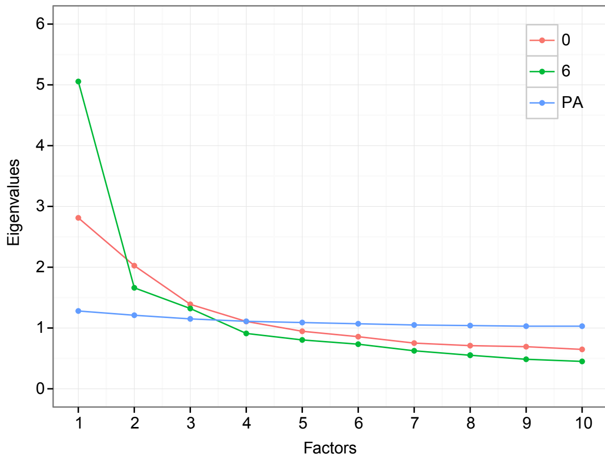
QIDS-C Eigenvalues at weeks 0 and 6
