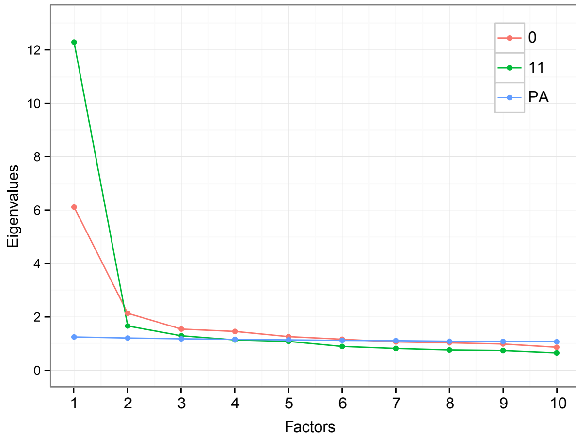
IDS-C Eigenvalues at weeks 0 and 11
