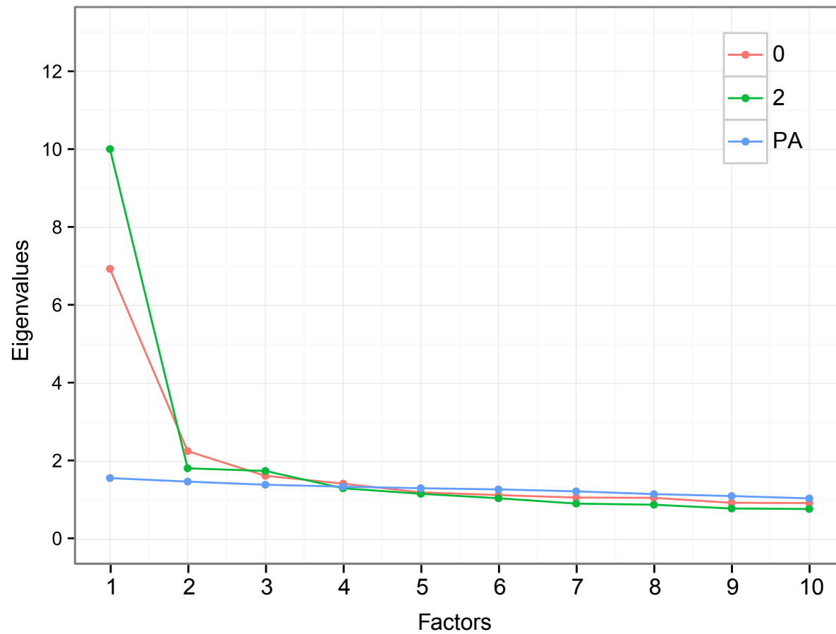
IDS-SR Eigenvalues at years 0 and 2
